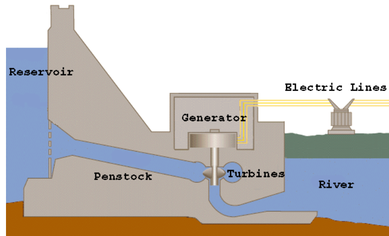
Figure 2: Diagram of a hydroelectric facility
