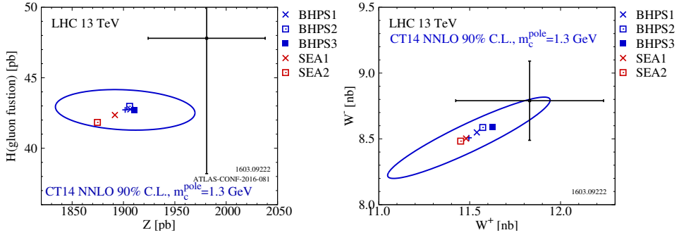
Figure 2. CT14 NNLO H (gluon-gluon fusion), Z , W^+ , and W^- production cross sections with an IC PDF component at the LHC \sqrt{s} = 13 TeV, with pole mass m_c^{pole} = 1.3 GeV. The 90% C.L. uncertainty regions for CT14 at NNLO and experimental points from ATLAS [23, 24] are also shown.
