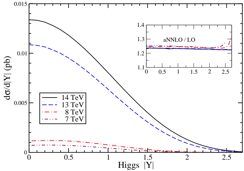
Figure 7: The aNNLO charged Higgs rapidity distributions for b\bar{b} \rightarrow H^- W^+ at the LHC with \sqrt{S} = 7, 8, 13, and 14 TeV, and m_H = 500 GeV.
