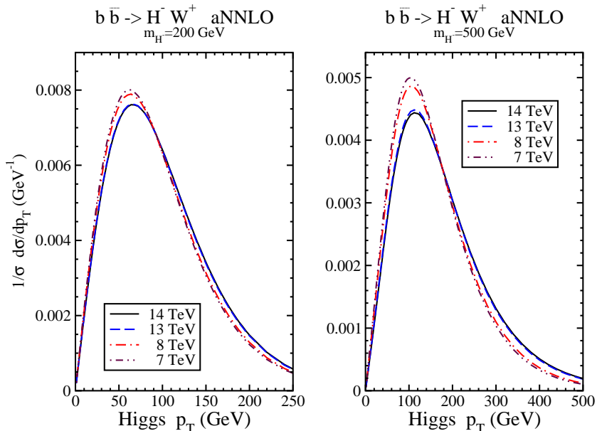
Figure 5: The aNNLO charged Higgs normalized p_T distributions for b\bar{b} \rightarrow H^-W^+ at the LHC with \sqrt{S} = 7, 8, 13, and 14 TeV, and m_H = 200 GeV (left) and 500 GeV (right).
