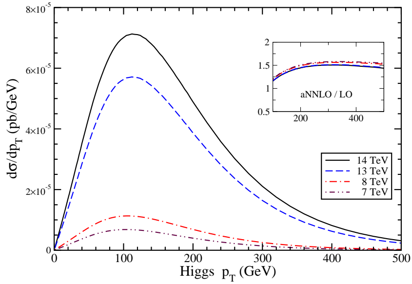
Figure 4: The aNNLO charged Higgs p_T distributions for b\bar{b} \rightarrow H^- W^+ at the LHC with \sqrt{S} = 7, 8, 13, and 14 TeV, and m_{H^-} = 500 GeV.
