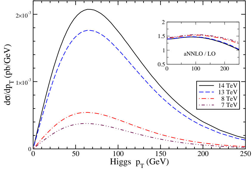
Figure 3: The aNNLO charged Higgs p_T distributions for b\bar{b} \rightarrow H^- W^+ at the LHC with \sqrt{S} = 7, 8, 13, and 14 TeV, and m_{H^-} = 200 GeV.
