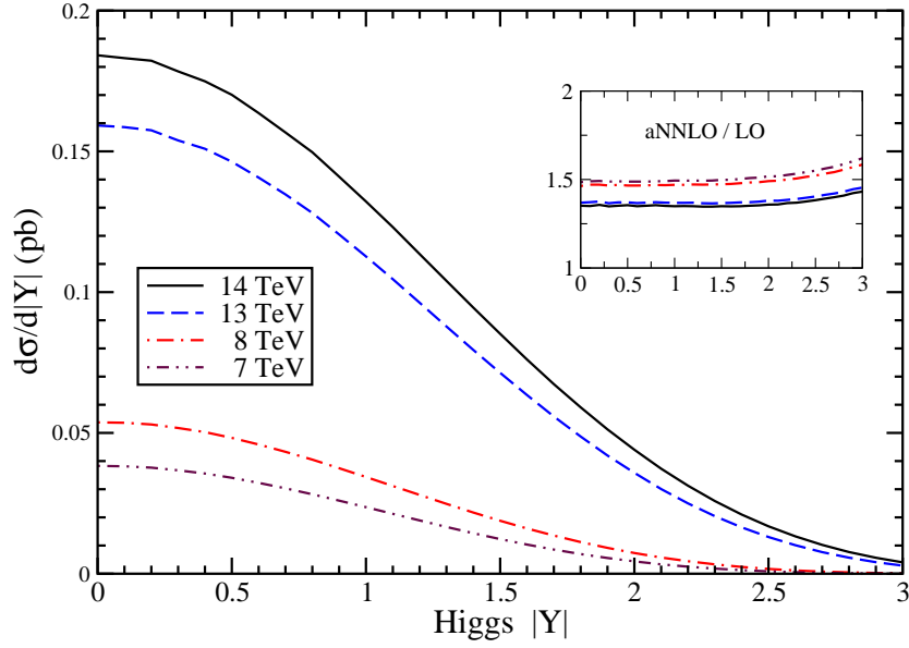
Figure 6: The aNNLO charged Higgs rapidity distributions for b\bar{b} \rightarrow H^- W^+ at the LHC with \sqrt{S} = 7, 8, 13, and 14 TeV, and m_H = 200 GeV.
