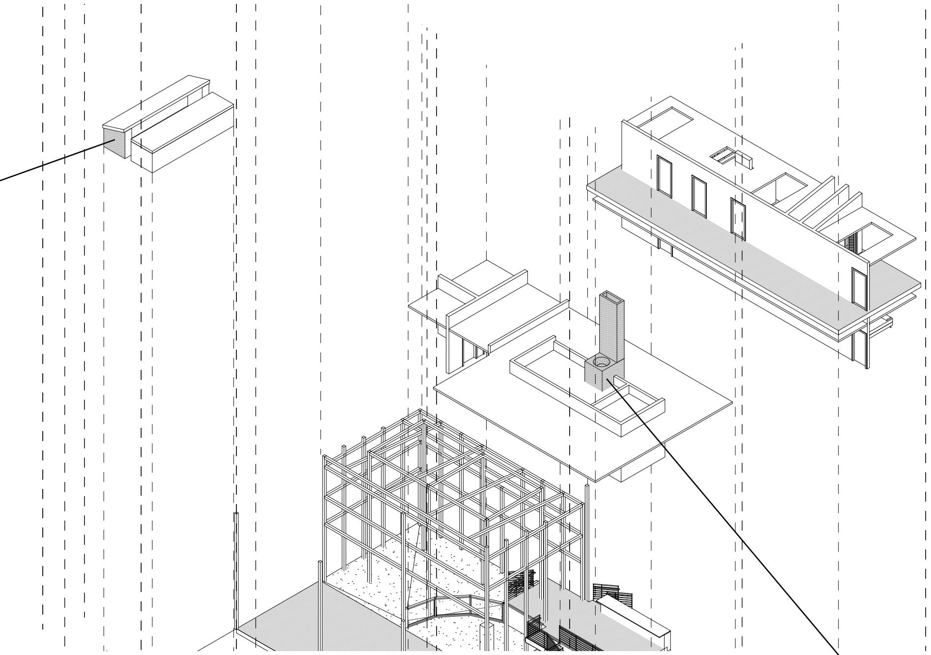
AXON: FIRST FLOOR INTERIOR
