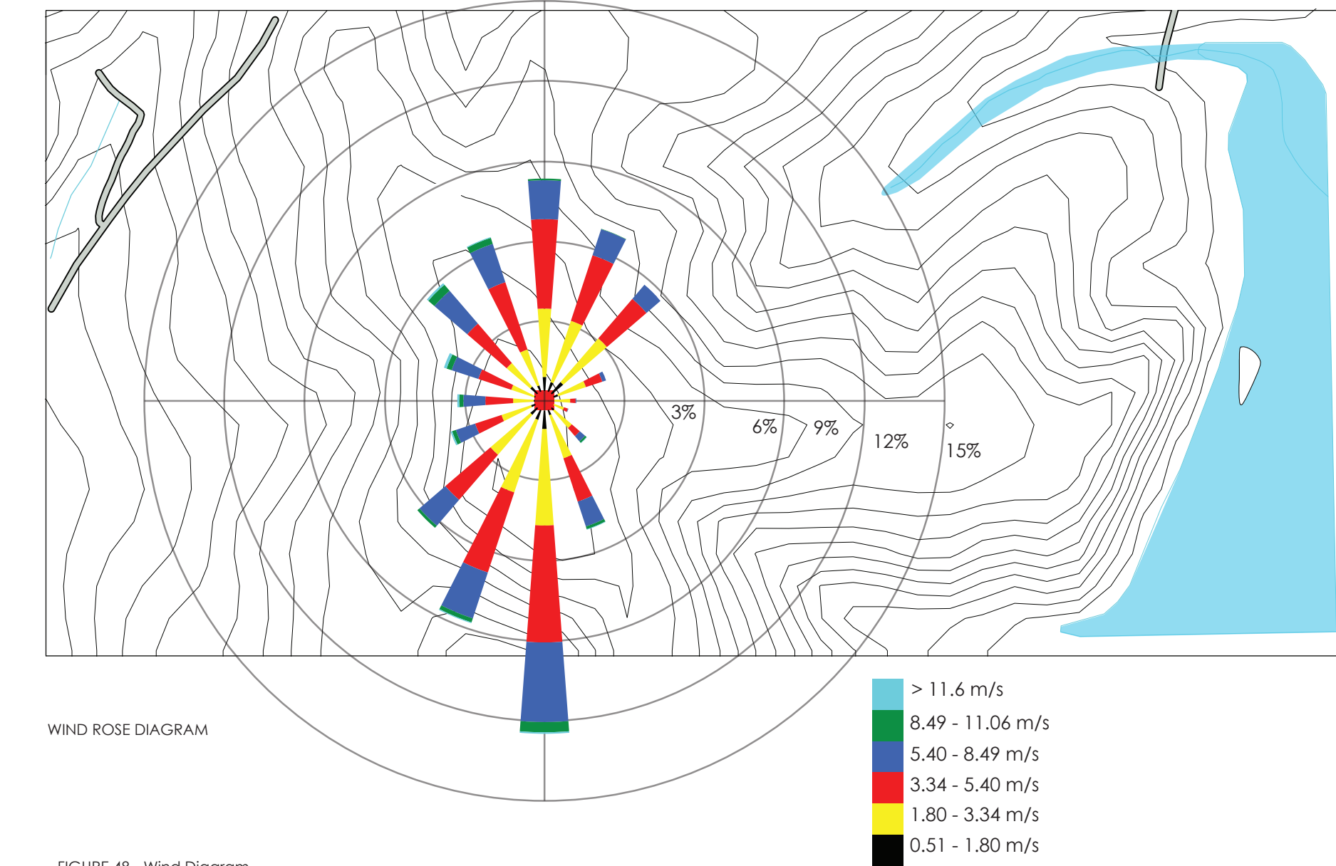
FIGURE 48 - Wind Diagram
