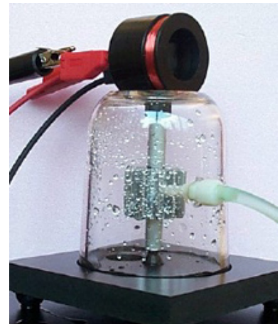
Figure 3: Turbine Generator
